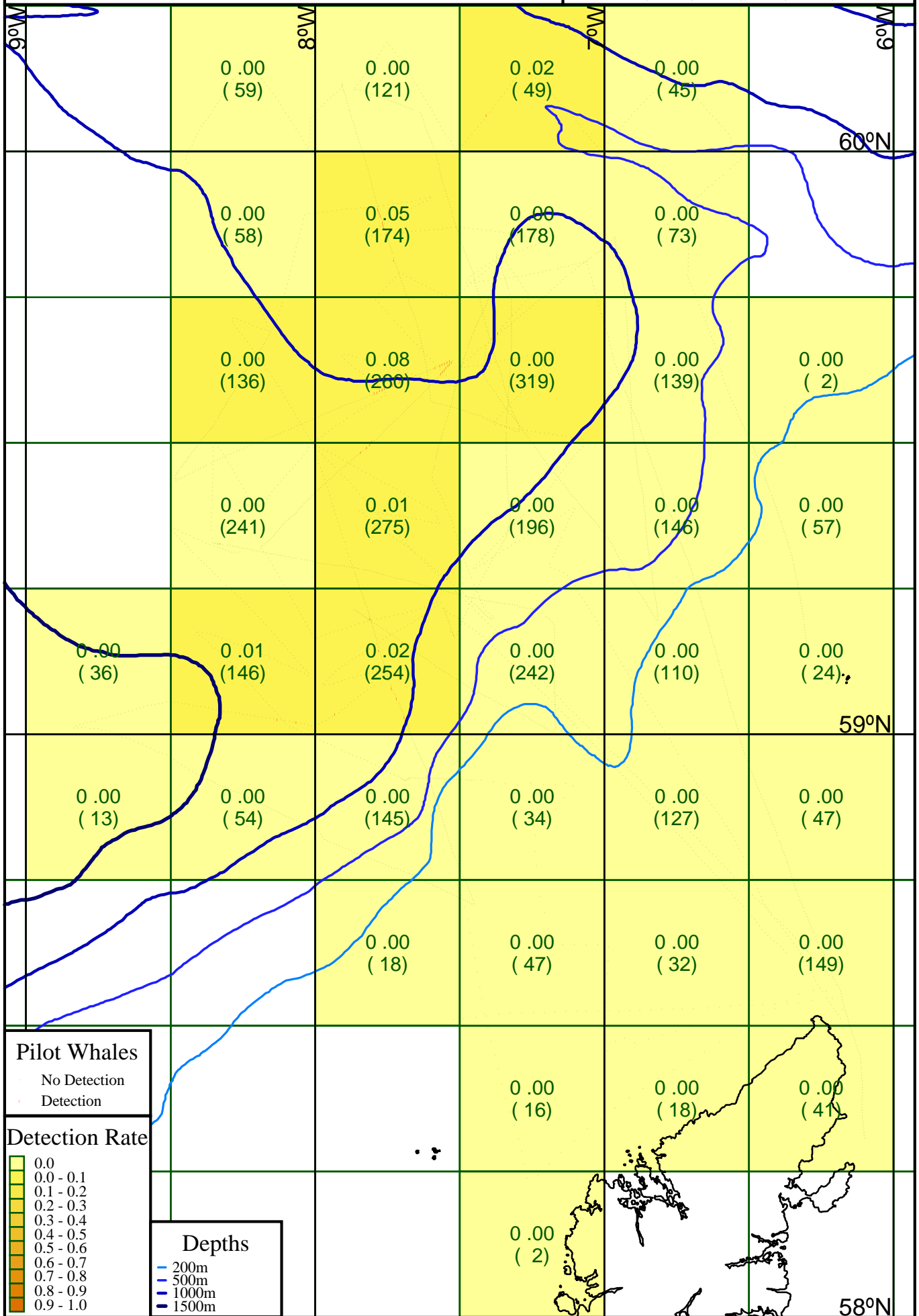
Chart 17 - Pilot Whale Detections - January
